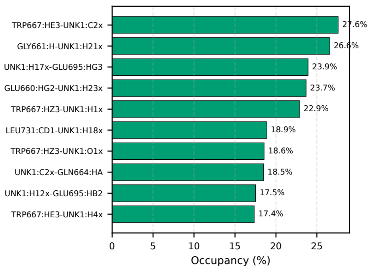
C: BMS-986205 / WT (Success)
